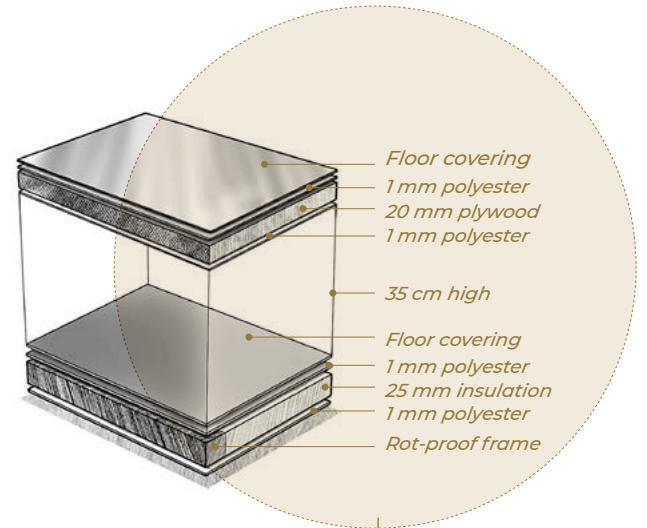
Diagram of the double floor
